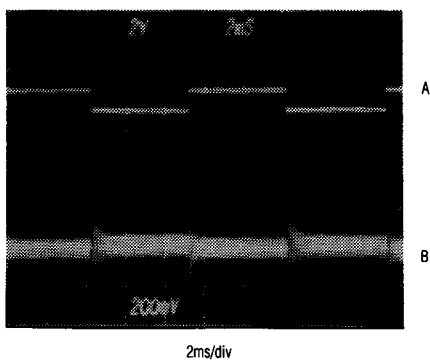
LINE-TRANSIENT RESPONSE
