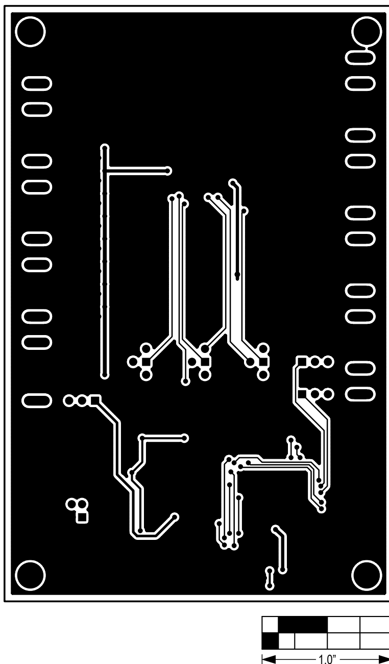
Figure 6. MAX7311 EV Kit PCB Layout—Solder Side
