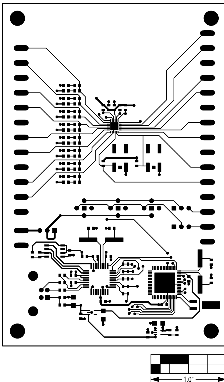
Figure 5. MAX7311 EV Kit PCB Layout—Component Side
