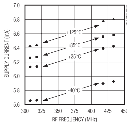
SUPPLY CURRENT vs. RF FREQUENCY (1x I_{LNA} )
