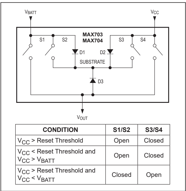
Figure 3. Battery-Switchover Block Diagram
