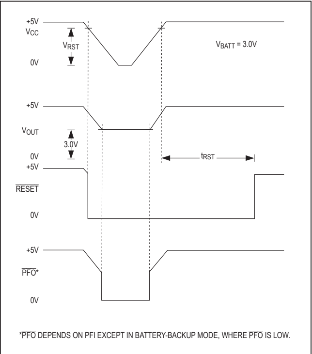
Figure 2. Timing Diagram
