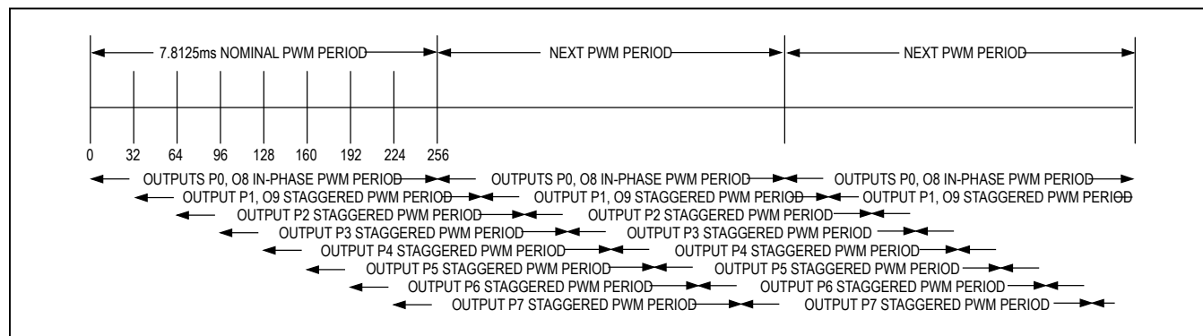
Figure 3. Stagqered PWM Waveform
