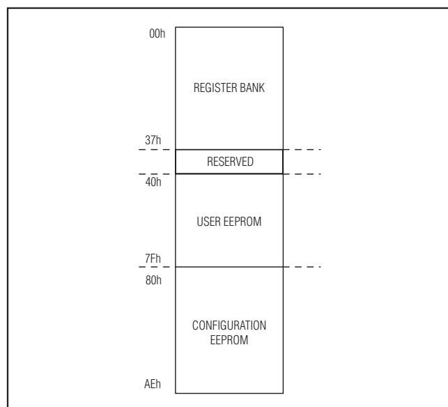
Figure 2. Memory Map
