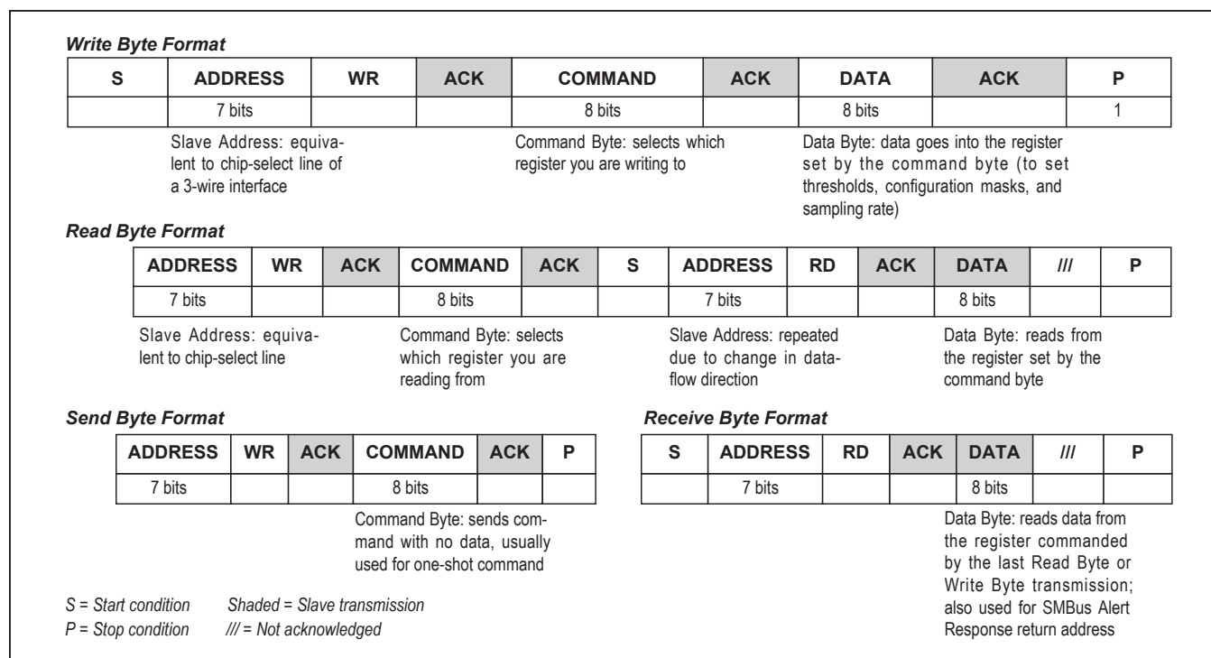
Figure 2. SMBus Protocols
