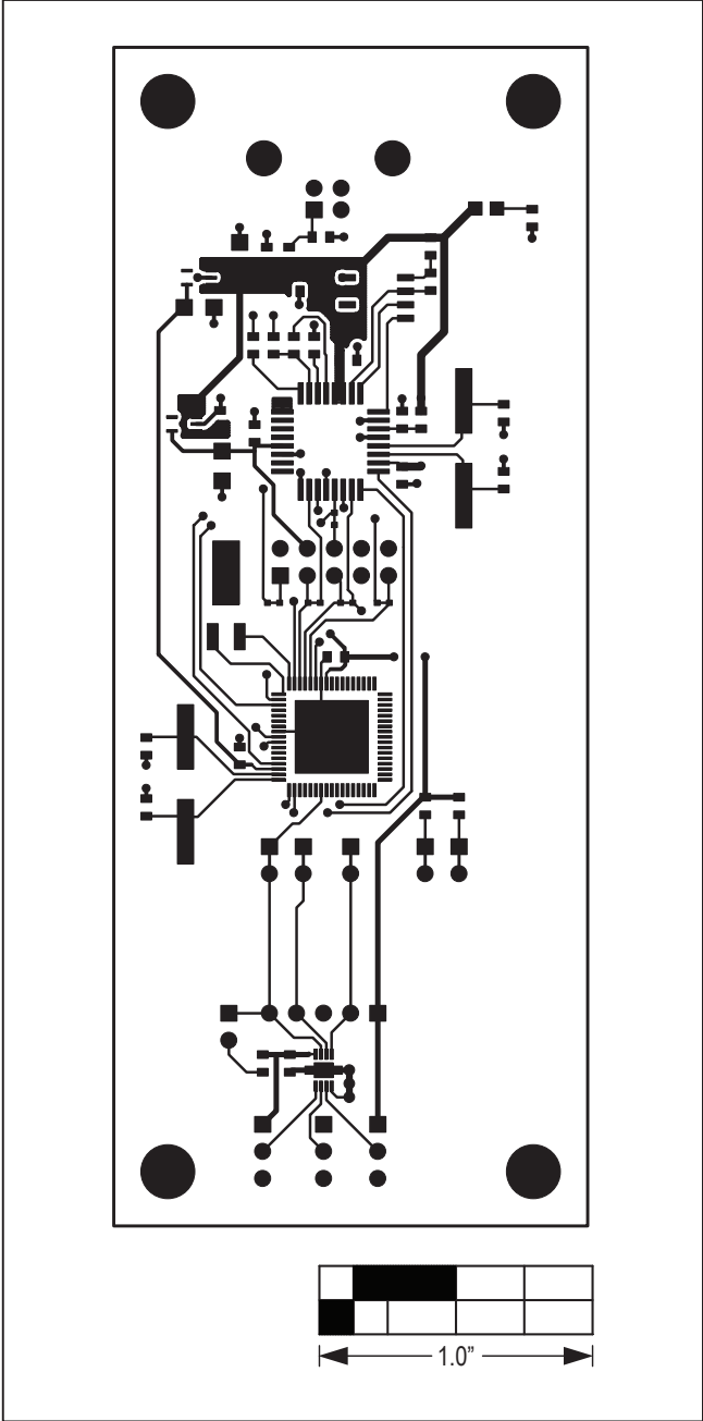
Figure 5. MAX6604 EV Kit PCB Layout—Component Side
