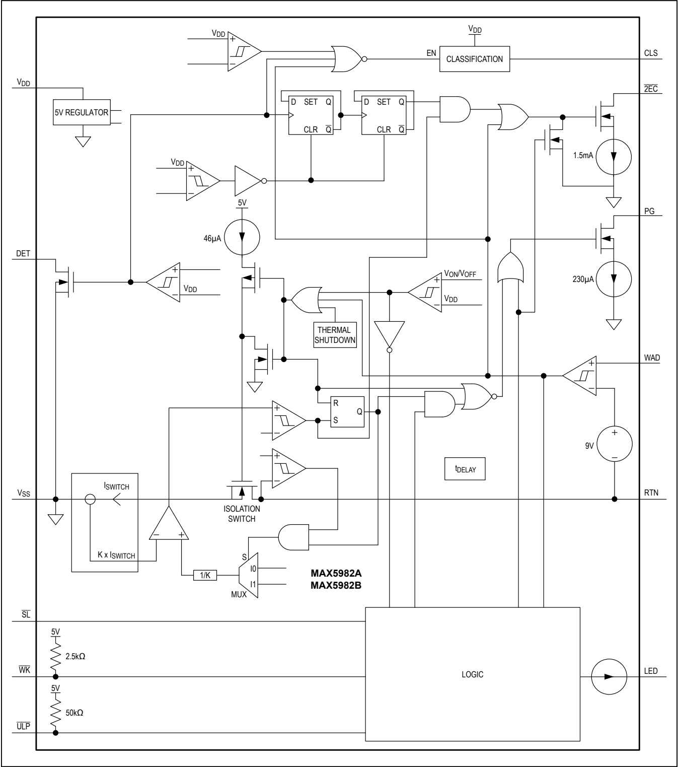
MAX5982A/MAX5982B Simplified Block Diagram
