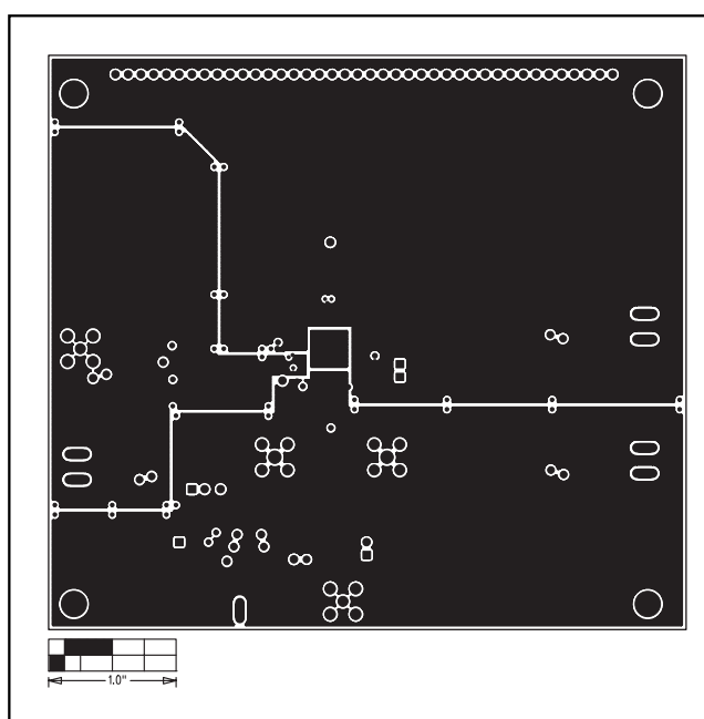
Figure 7. MAX5886/MAX5887/MAX5888 EV Kit PC Board Layout—Power Planes
