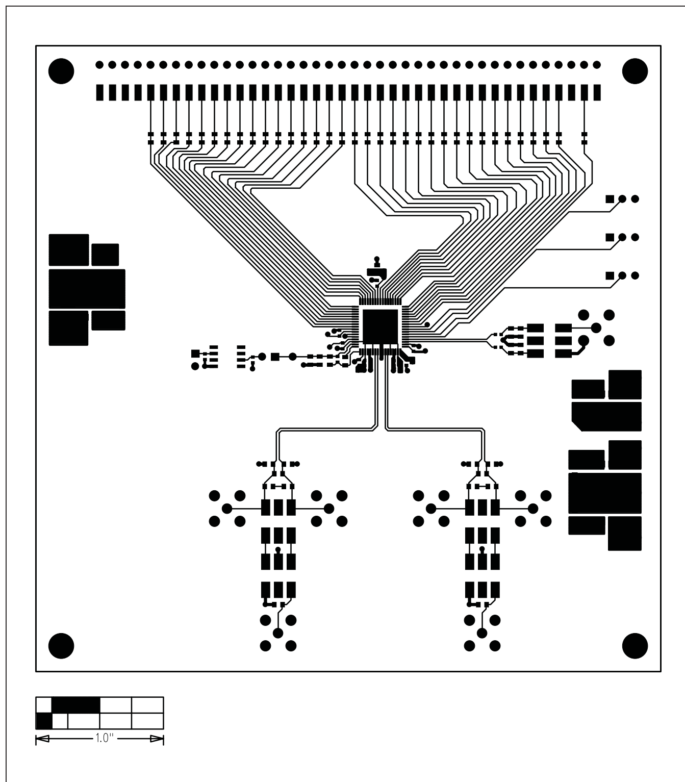
Figure 6. MAX5873/MAX5874/MAX5875 EV Kit PC Board Layout—Component Side (Layer 1)
