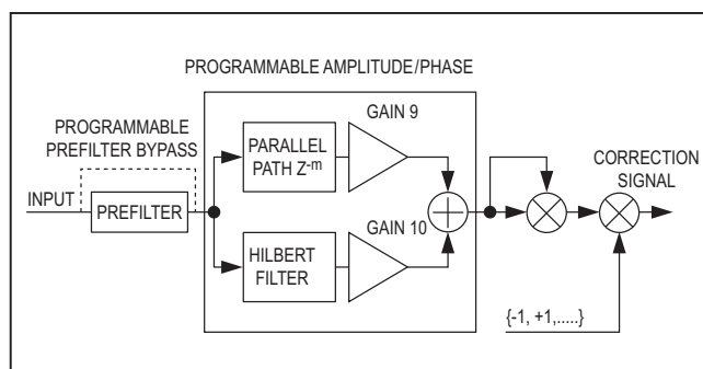
Figure 15. f_{DAC}/2 - 2 \times f_{OUT} DAC DPD
