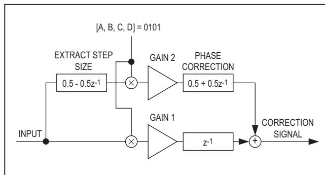
Figure 13. DAC Interleaving Error Compensation Block Diagram
