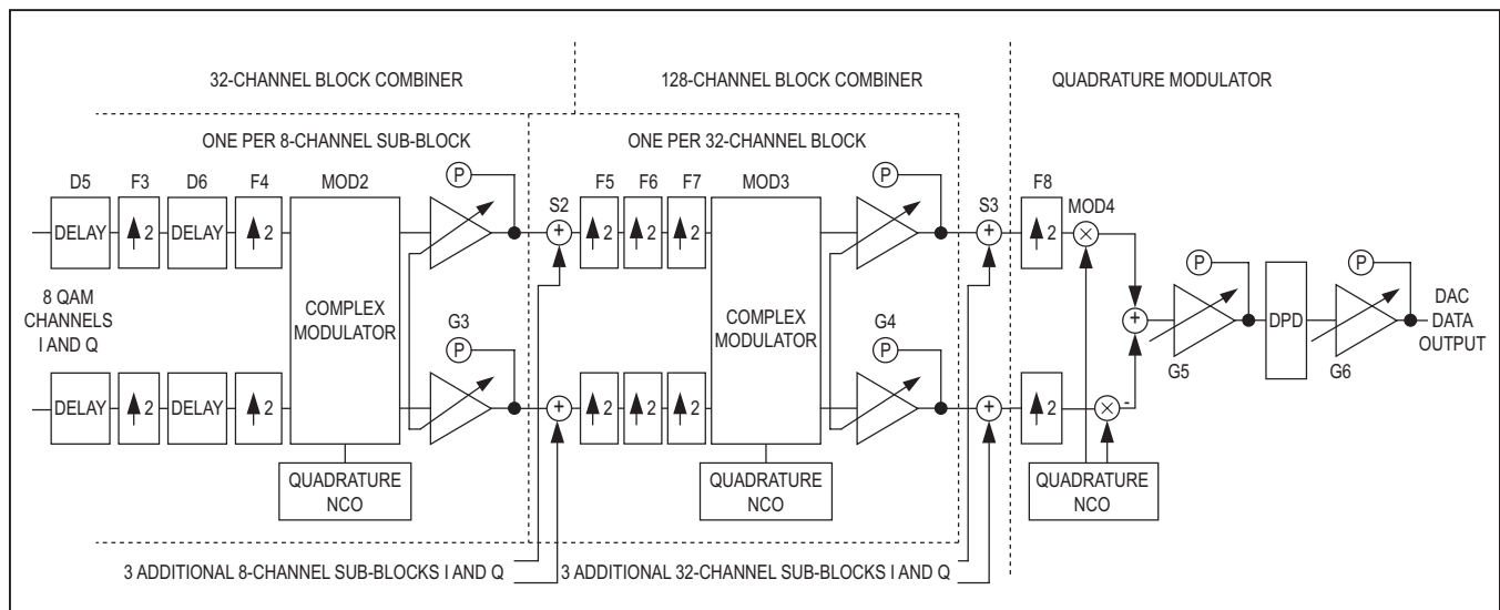
Figure 10. Channel Combiners and Interpolation/Modulation
