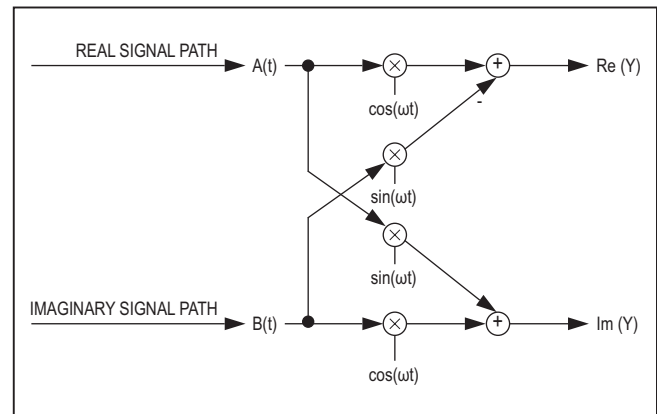
Figure 11. Complex Modulator Block Diagram
