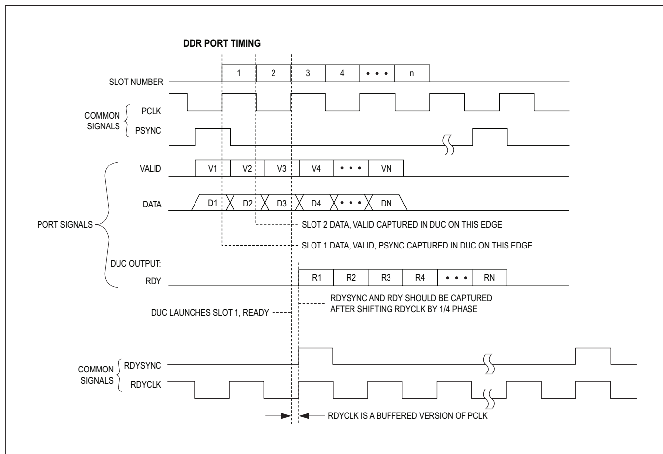
Figure 8. Example of Port Timing Diagram (DDR)
