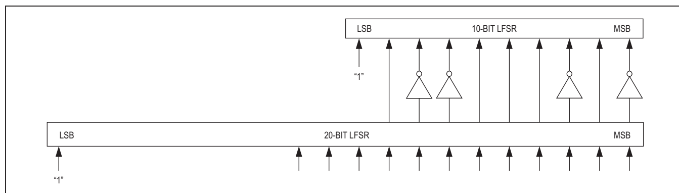
Figure 24. LFSR Seeds
