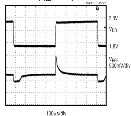
REFERENCE LINE-TRANSIENT RESPONSE ( V_{REF} = 1.2V )
