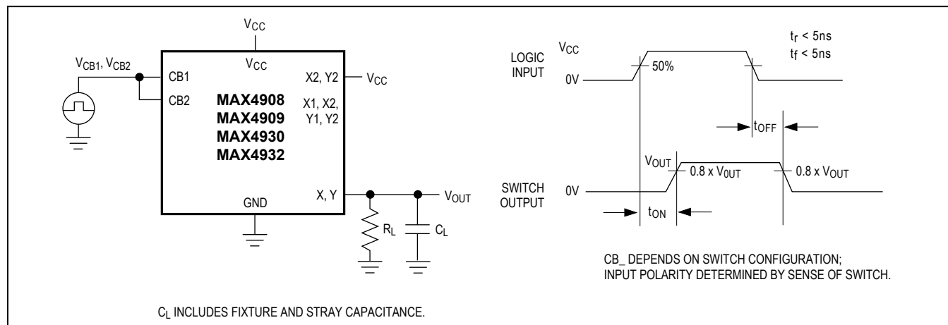
Figure 2. Switching Time
