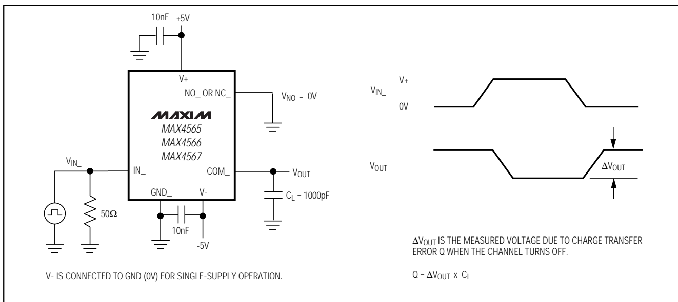
Figure 5. Charge Injection
