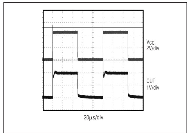
Figure 6. Power-Up/Power-Down Waveform
