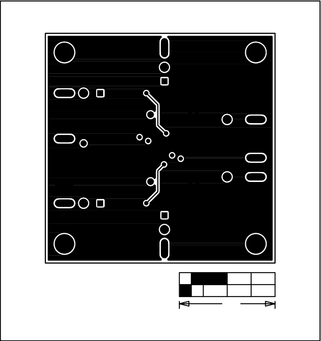
Figure 4. MAX44246 EV Kit PCB Layout—Solder Side
