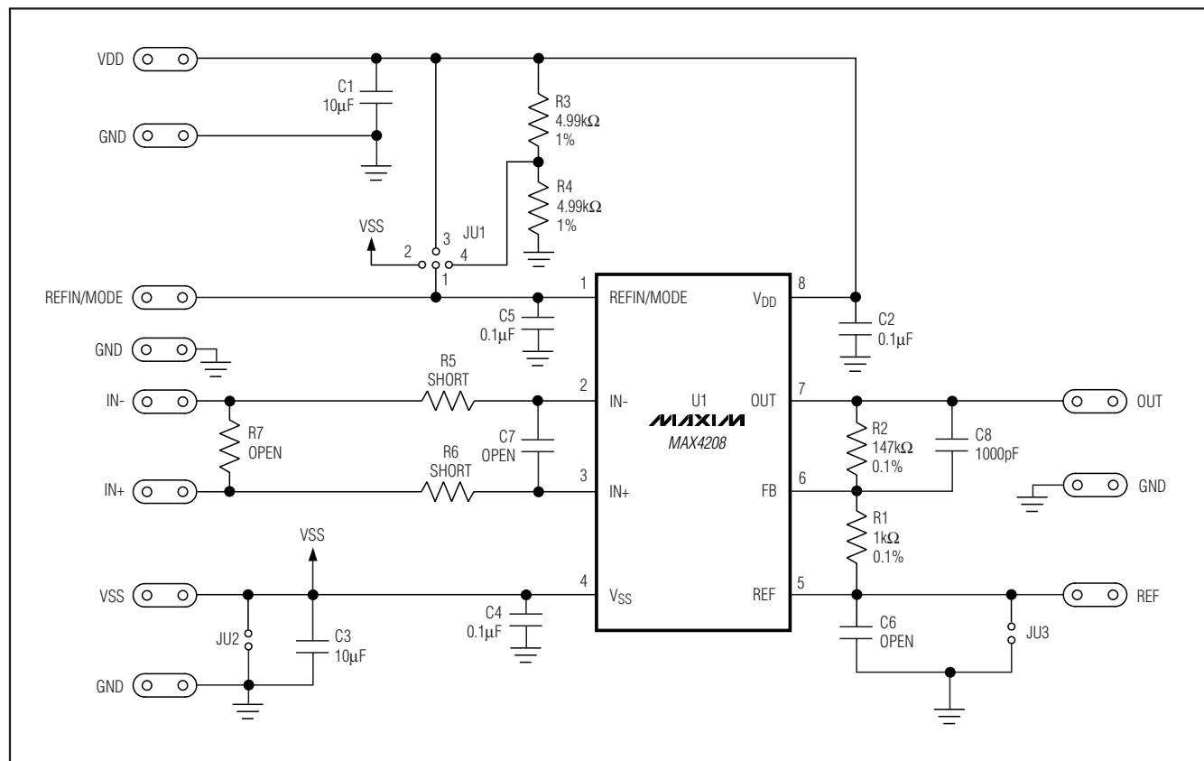
Figure 1. MAX4208 EV Kit Schematic
