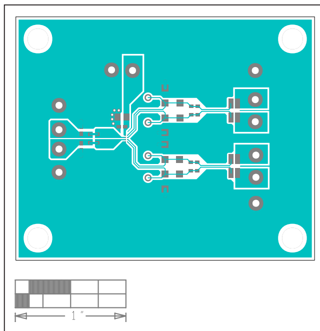
MAX40201 EV Kit PCB Layout—Top
