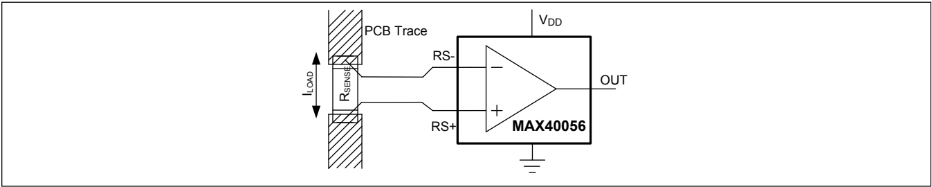
Figure 4. Kelvin Sensing
