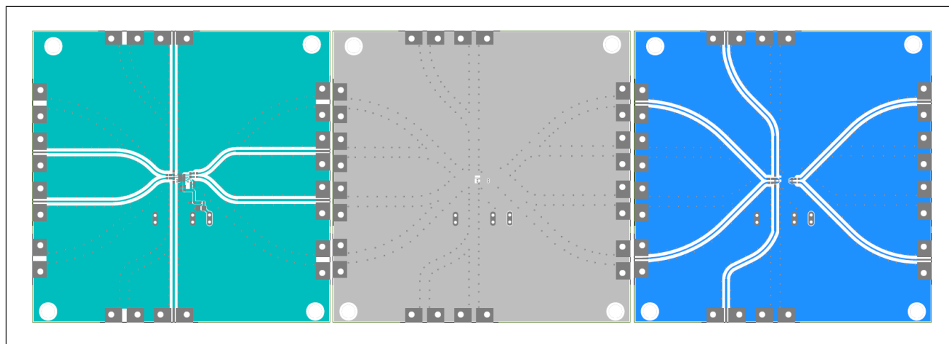
Figure 7. Layout Guidelines—Ground Keep-Out to Avoid Stubs.
