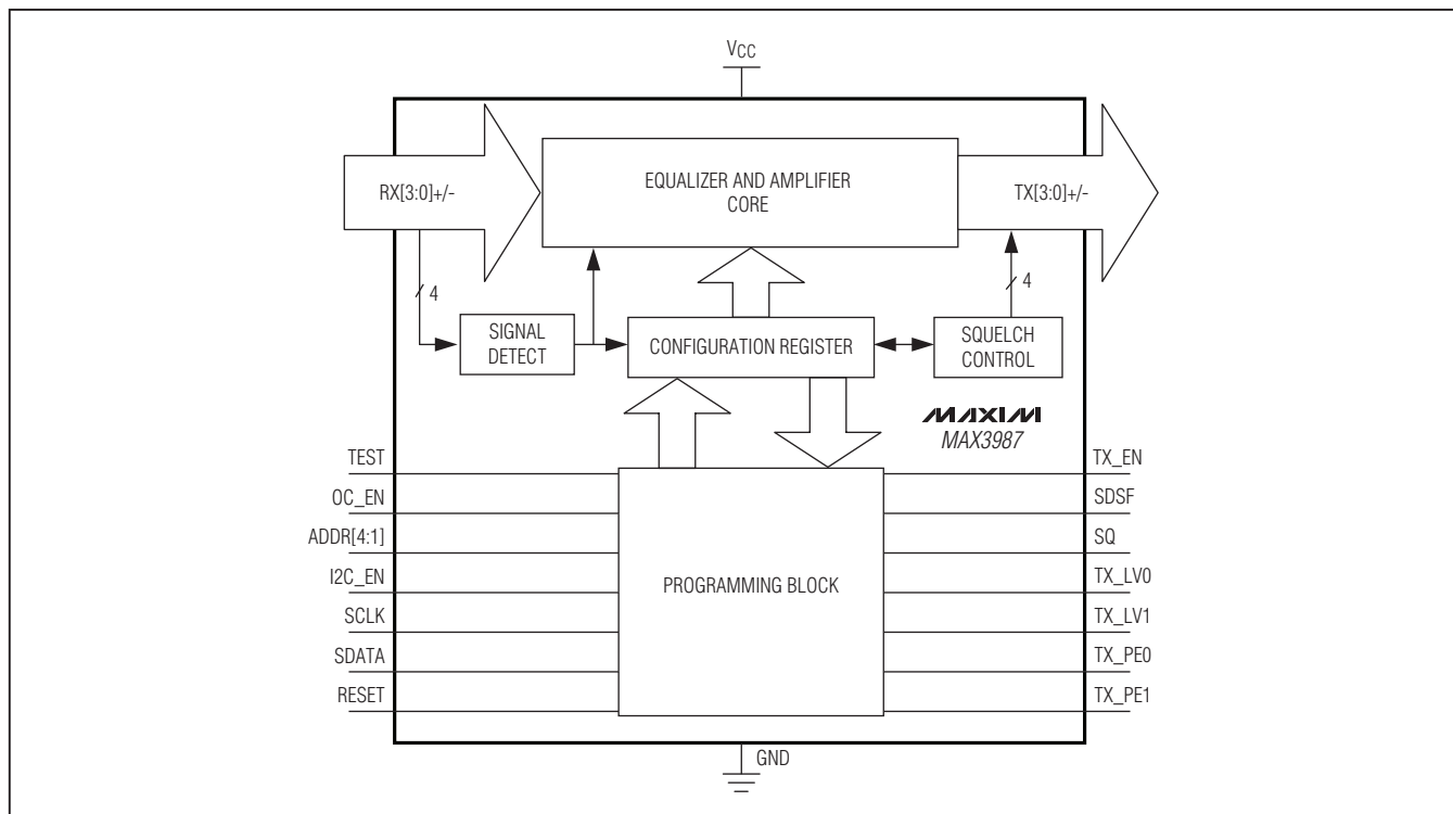
Figure 5. Functional Diagram
