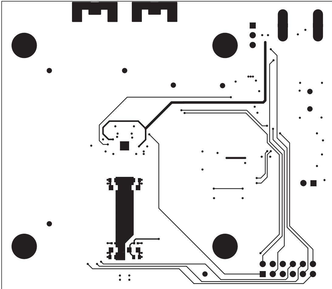
Figure 8. MAX3946 EV Kit PCB Layout—Solder Side
