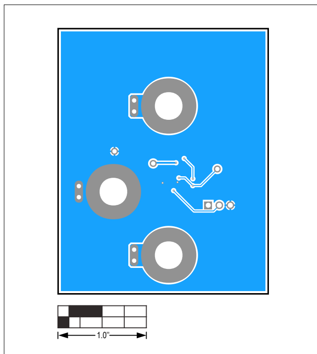
MAX38902E EV Kit—Bottom View
