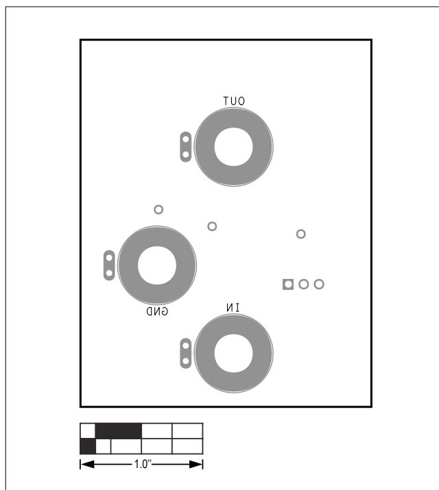
MAX38902E EV Kit—Bottom Silkscreen
