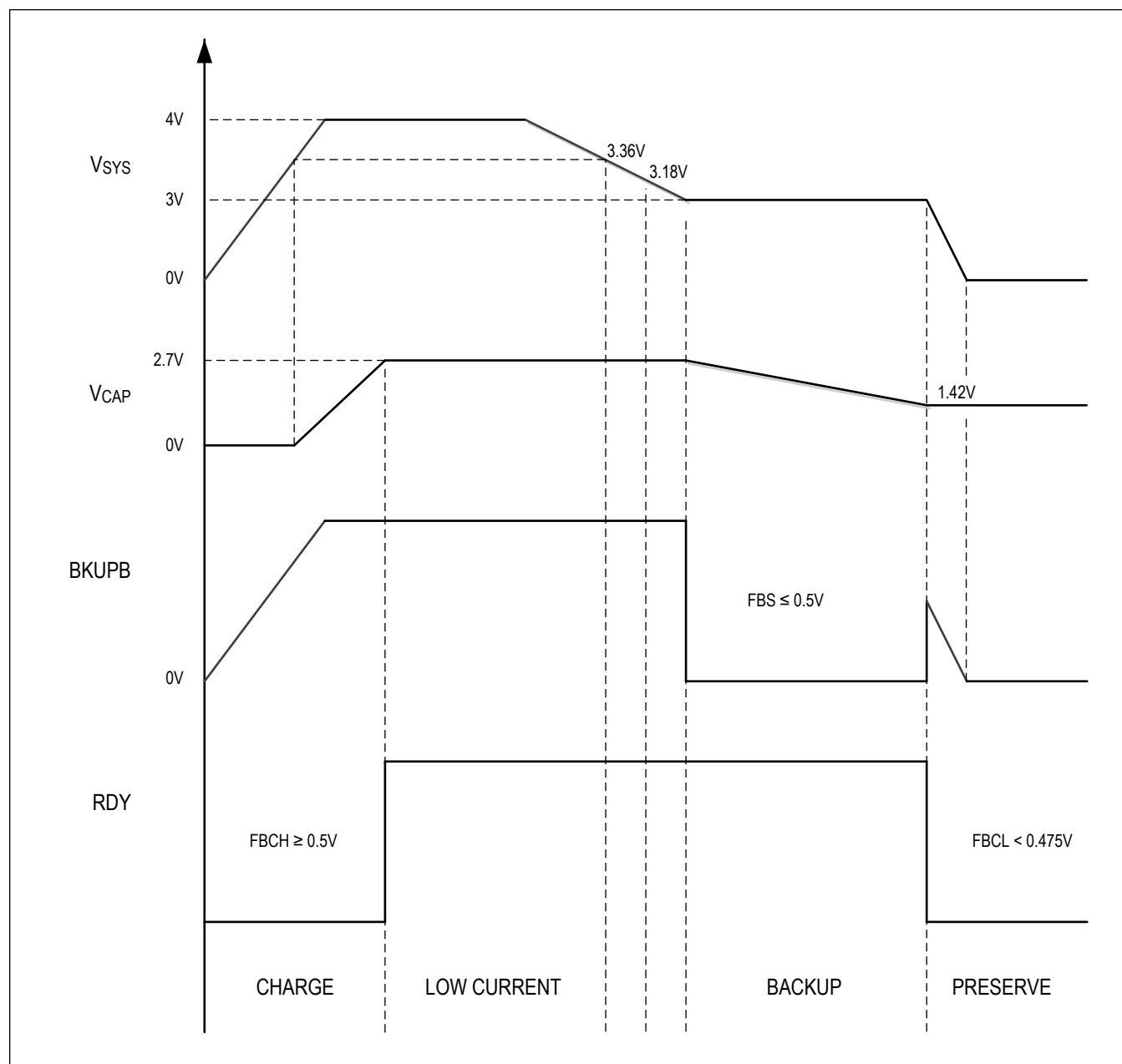
Figure 2. System Waveforms
