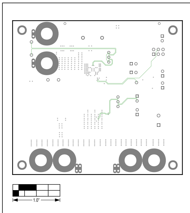
MAX38803 EV Kit—Internal 3
