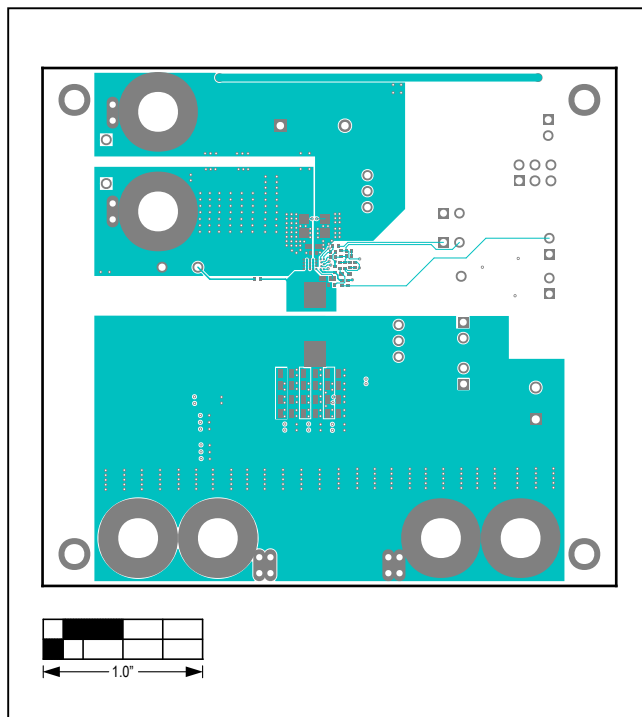
MAX38803 EV Kit—Top
