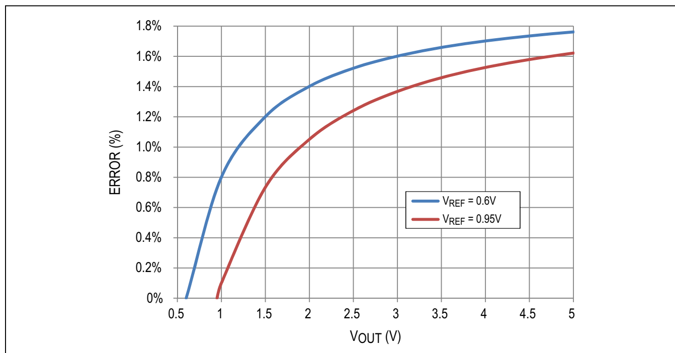
Figure 5. Contribution of 1% Tolerance Resistors on V_{OUT} Error
