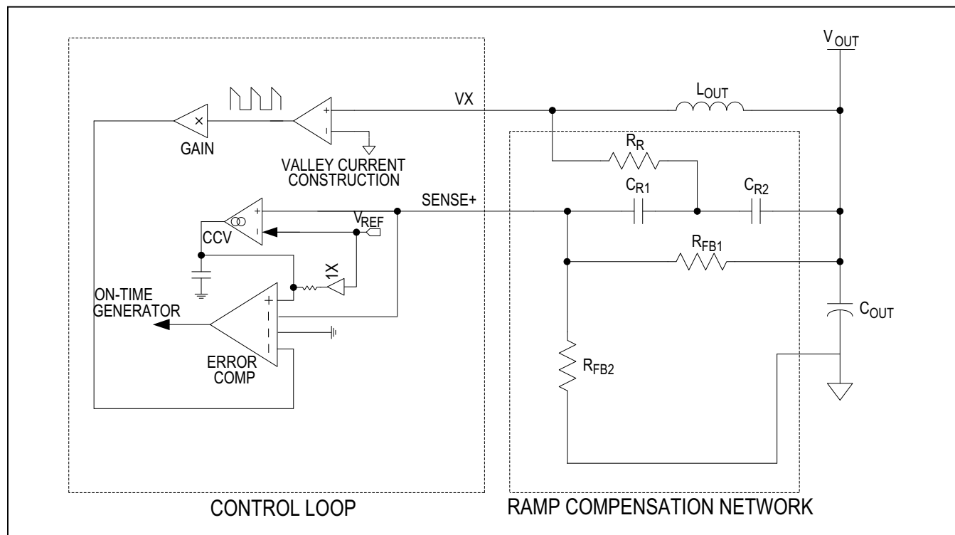
Figure 7. Ramp Compensation Diagram
