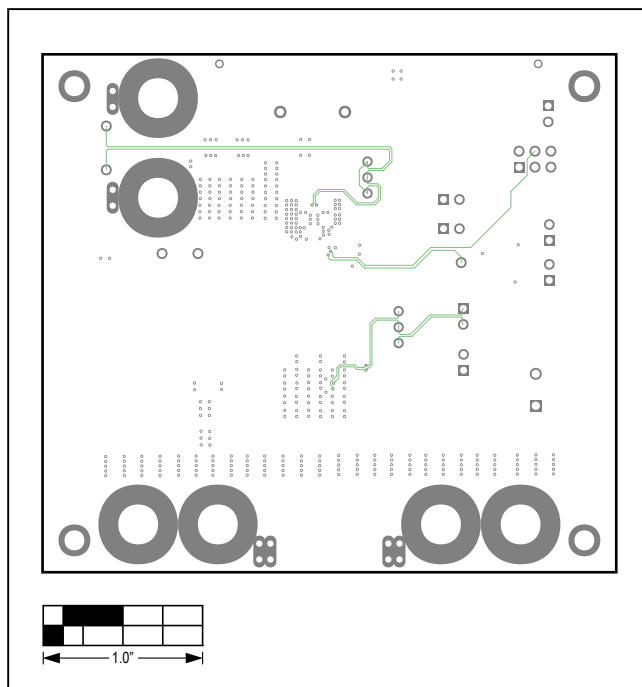
MAX38802 EV Kit—Internal 3
