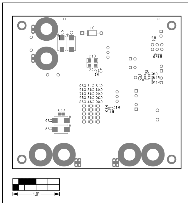
MAX38802 EV Kit—Bottom Silkscreen
