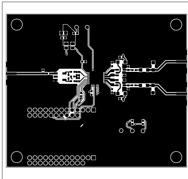
MAX3522B EV Kit—Top
