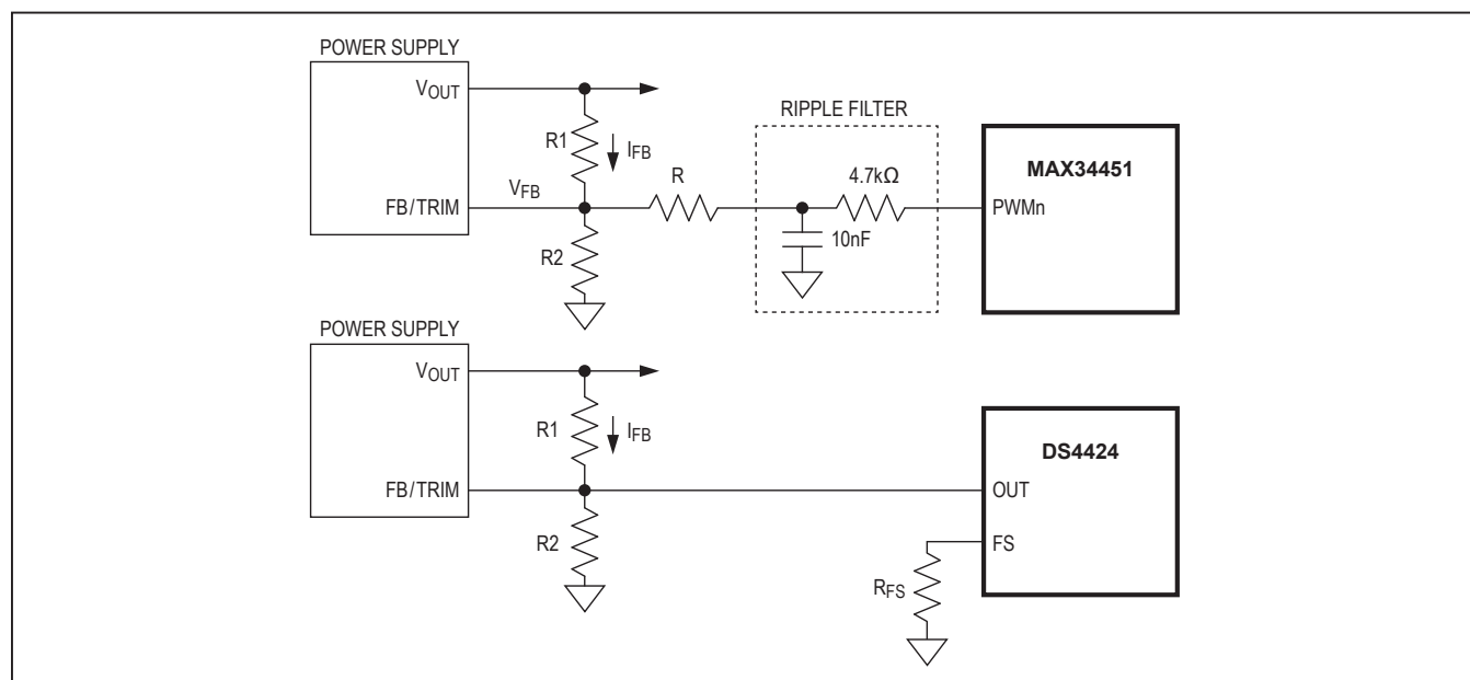
Figure 14. Margining Hardware Configurations
