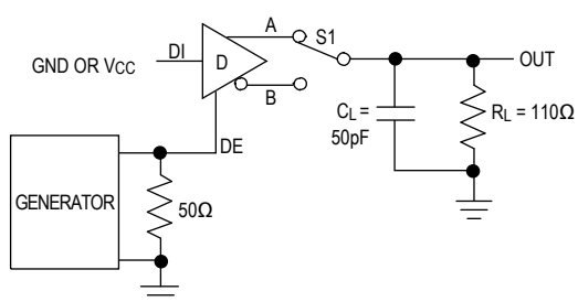
Figure 4. Driver Enable and Disable Times ( t_{DZH} , t_{DHZ} )
