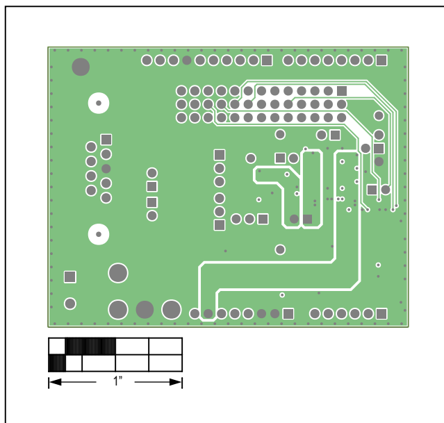
MAX33012E Shield—Internal 3
