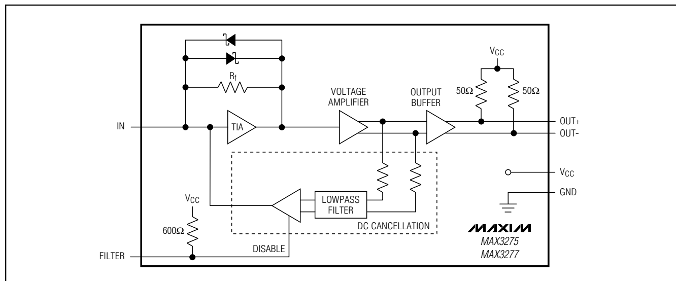
Figure 1. Functional Diagram
