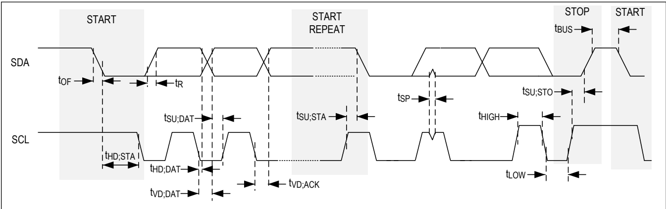
Figure 3. I²C Timing Diagram
