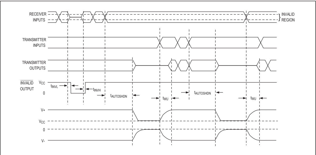
Figure 3b. AutoShutdown Plus, \overline{\text{INVALID}} , and READY Timing Diagram
