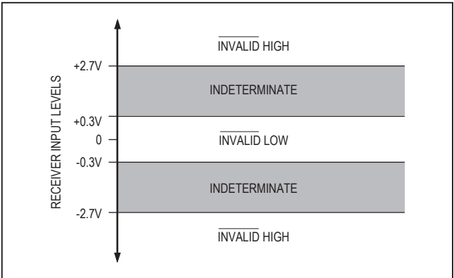
Figure 4a. Receiver Positive/Negative Thresholds for INVALID
