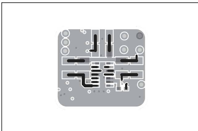
Figure 12. MAX30101 Daughter Board Component Placement Guide—Solder Side
