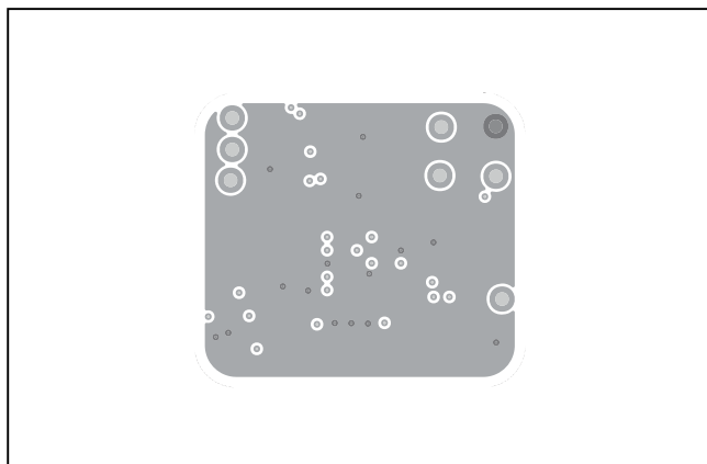
Figure 9. MAX30101 Daughter Board PCB Layout—Layer 3
