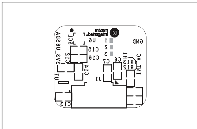
Figure 7. MAX30101 Daughter Board Component Placement Guide—Component Side
