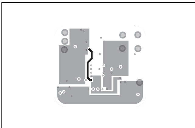
Figure 10. MAX30101 Daughter Board PCB Layout—Component Side
