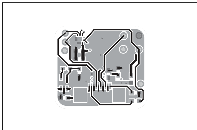
Figure 8. MAX30101 Daughter Board PCB Layout—Layer 2
