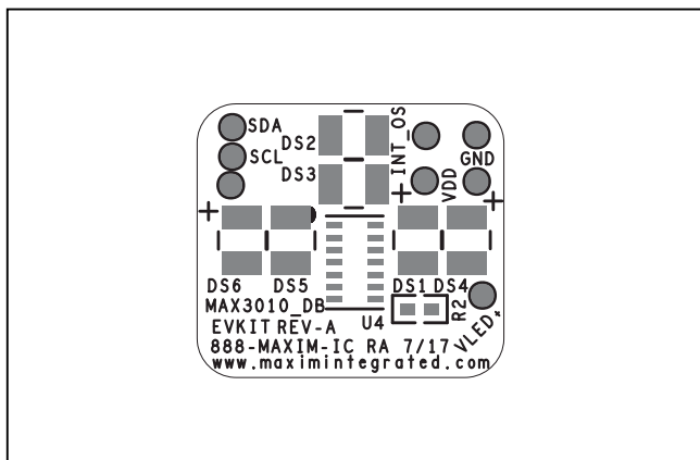
Figure 11. MAX30101 Daughter Board PCB Layout—Solder Side
