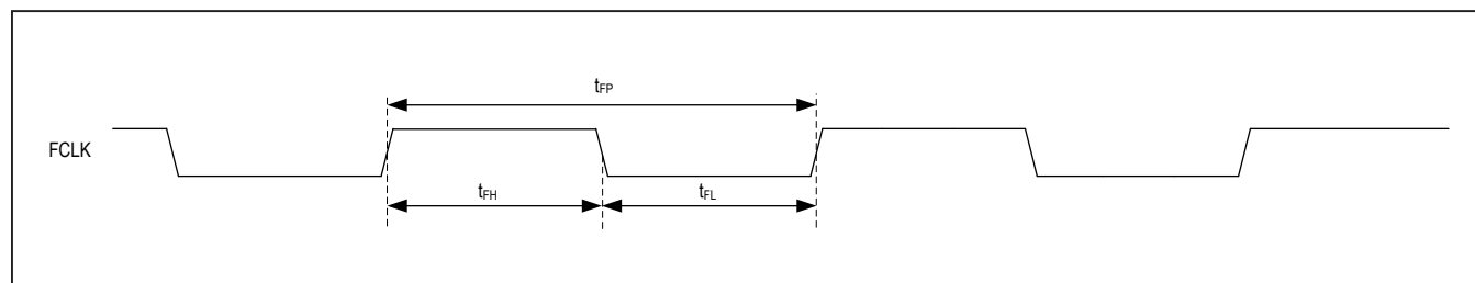
Figure 1b. FCLK Timing Diagram
