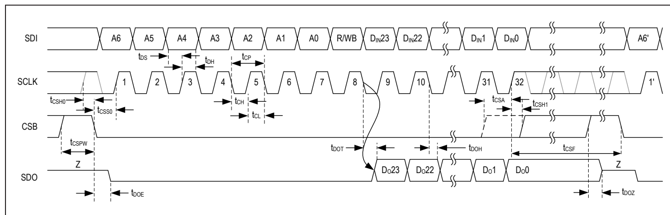
Figure 1a. SPI Timing Diagram
