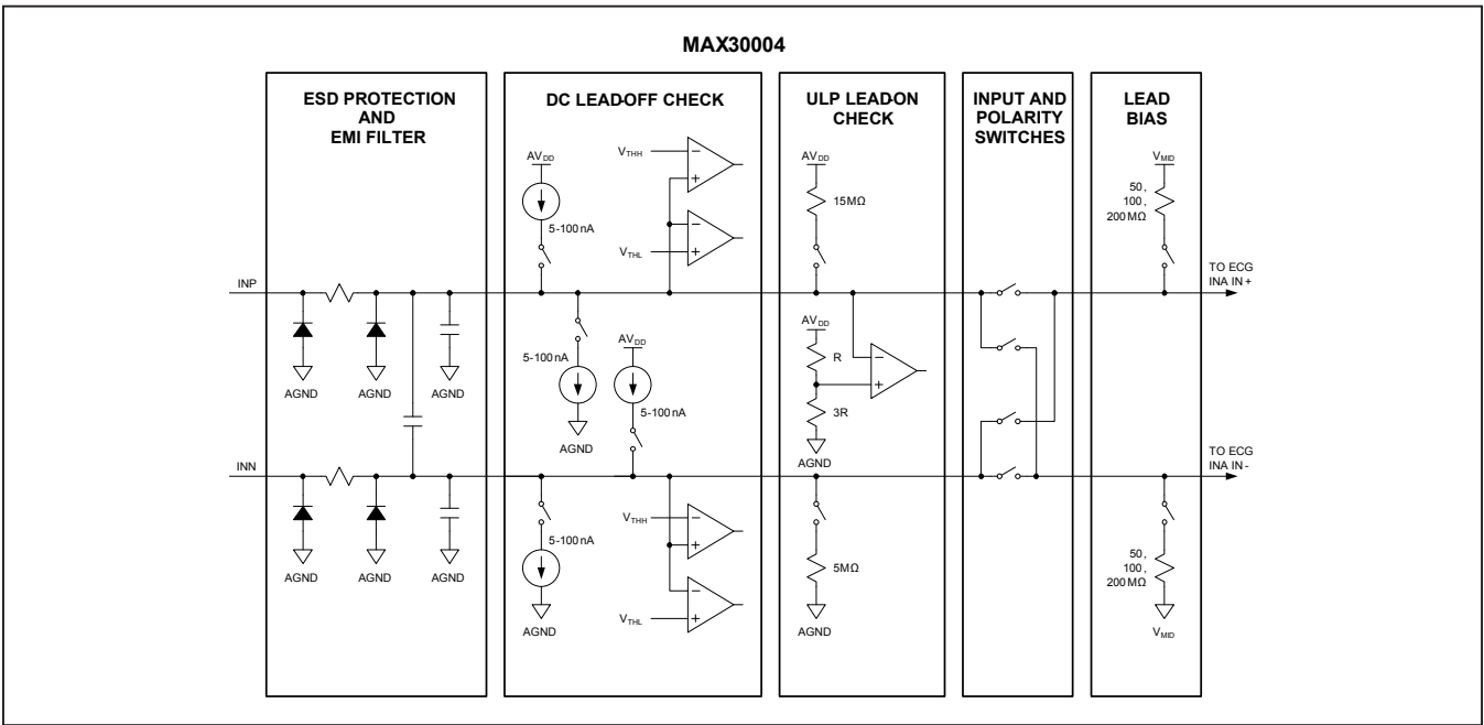
Figure 3. Input MUX
