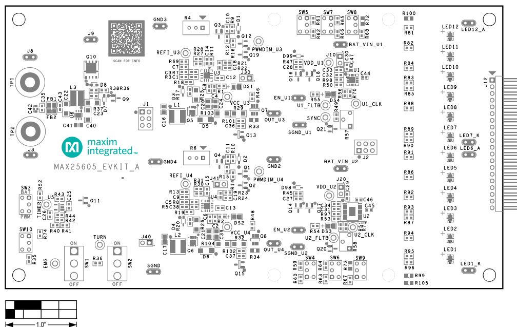
MAX25605 EV Kit PCB Layout—Top Silkscreen
