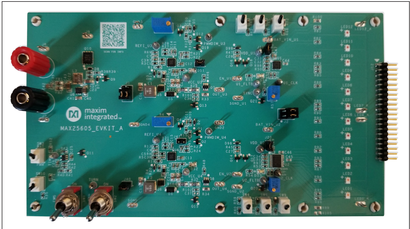
Figure 1. MAX25605EVKIT#
