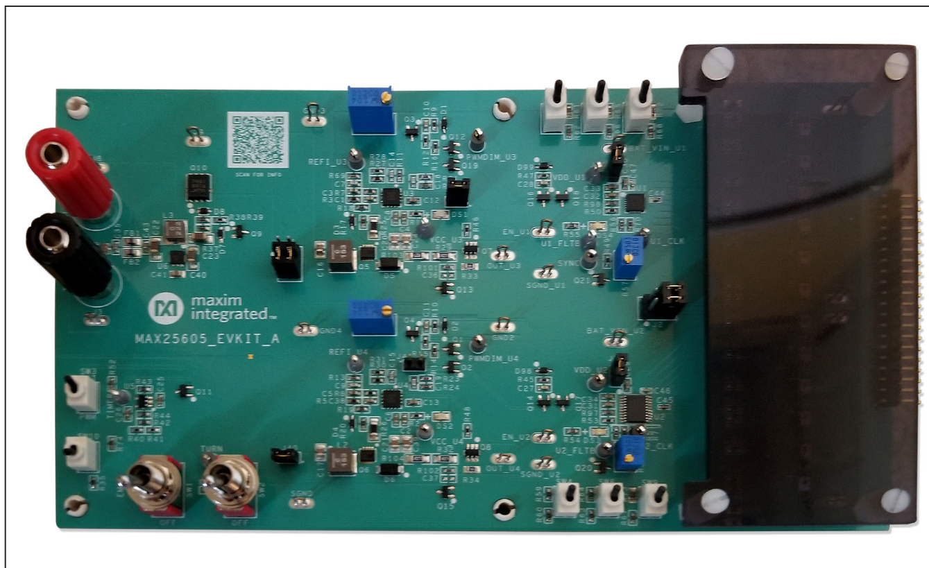
Figure 3. MAX25605EVKIT# with Acrylic Shield Installed
