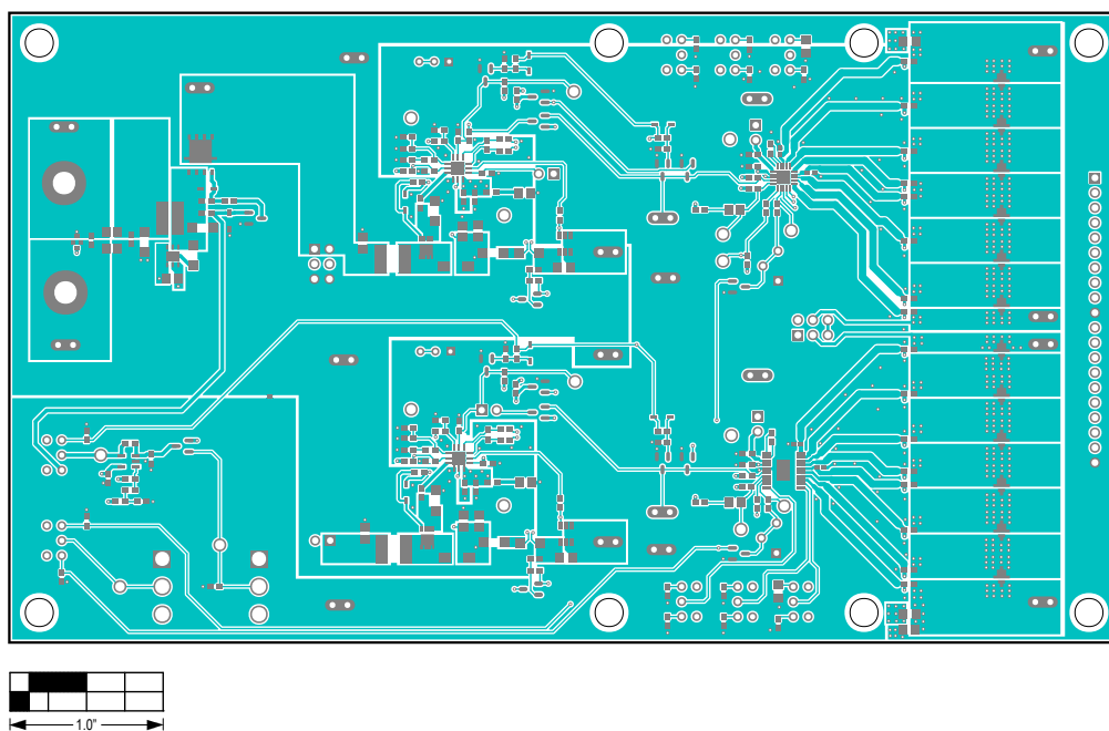
MAX25605 EV Kit PCB Layout—Top View
