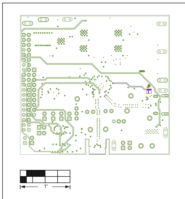
MAX25430A EV Kit PCB Layout - Layer 7
