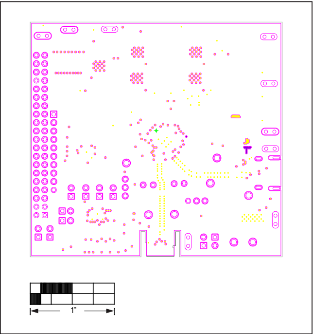
MAX25430A EV Kit PCB Layout - Layer 2
