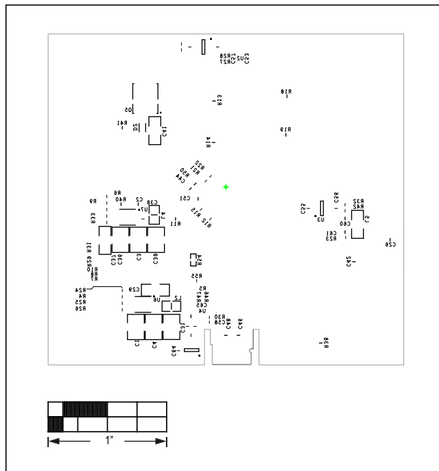
MAX25430A EV Kit PCB Layout - Bottom Silkscreen
