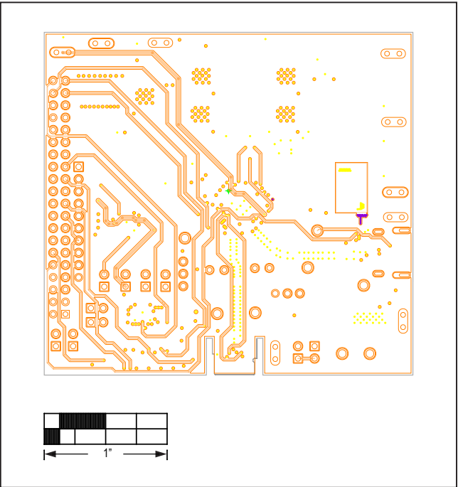
MAX25430A EV Kit PCB Layout - Layer 3
