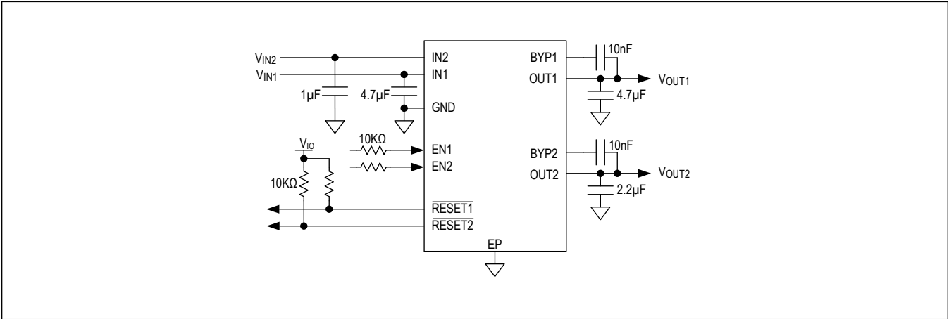
Circuit 2 (MAX25307)
