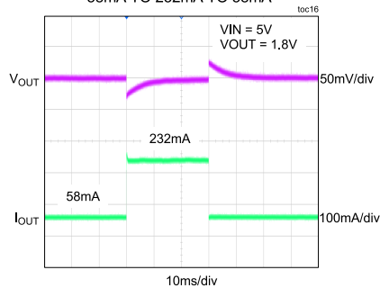
CH2 LOAD TRANSIENT RESPONSE 58mA TO 232mA TO 58mA
