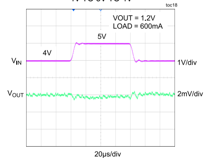
CH1 LINE TRANSIENT RESPONSE 4V TO 5V TO 4V
