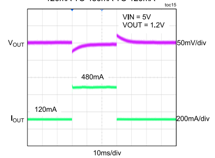
CH1 LOAD TRANSIENT RESPONSE 120mA TO 480mA TO 120mA
