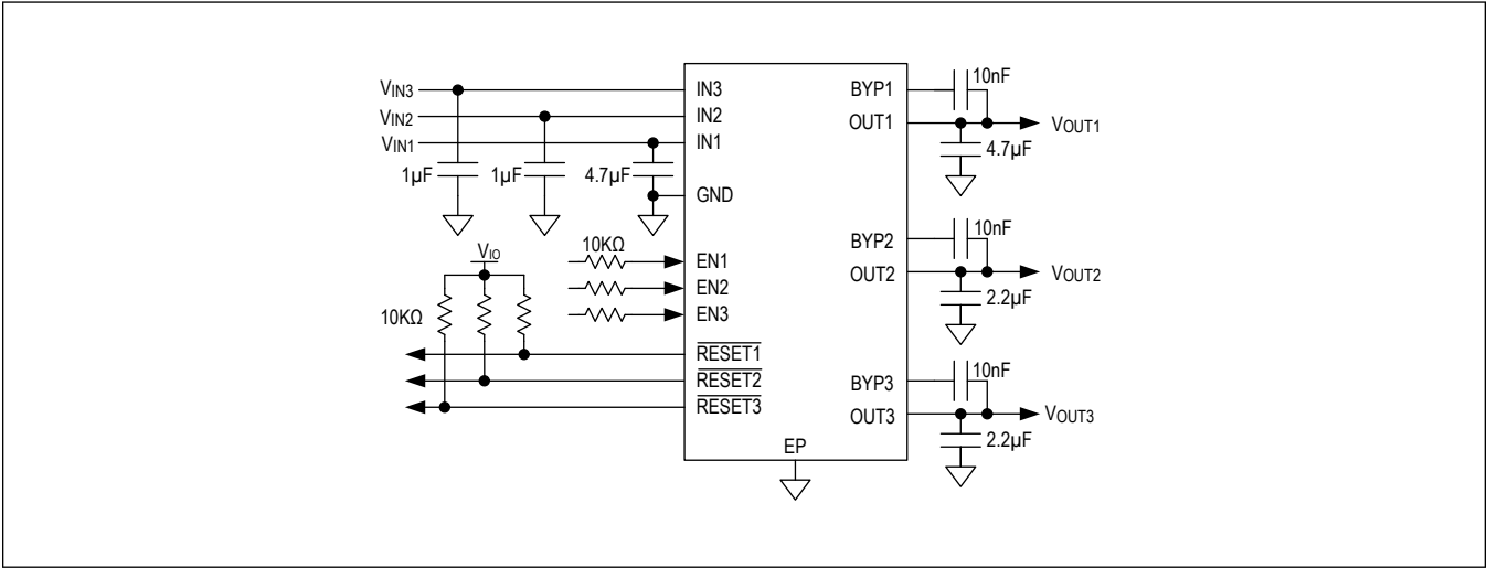
Circuit 2 (MAX25307)
