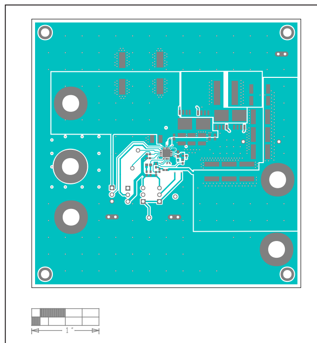
MAX25206/8 EVKit PCB Layout – Art Film – Top
