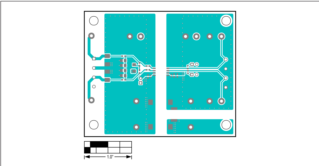
MAX22518 EV Kit PCB Layout—Top Layer
