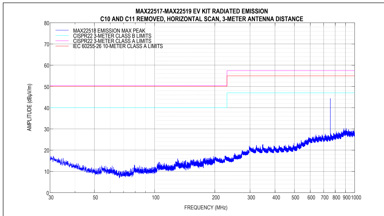
Figure 3. MAX22518 EV Kit Radiated Emission, Horizontal Scan
