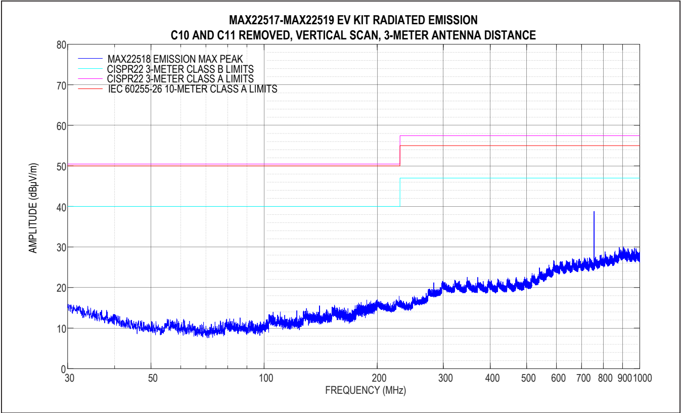
Figure 4. MAX22518 EV Kit Radiated Emission, Vertical Scan
