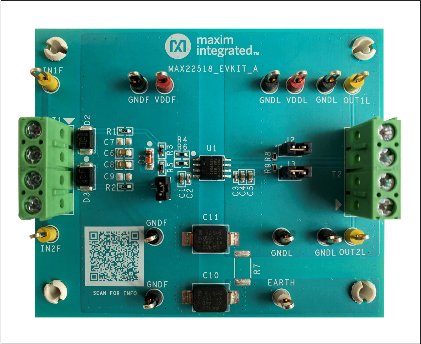
Figure 1. MAX22518EVKIT#
