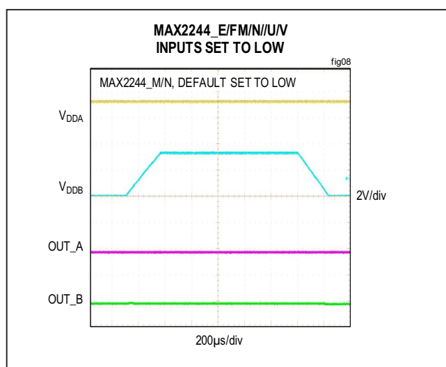
Figure 8. Undervoltage Lockout Behavior (MAX2244_Low)
