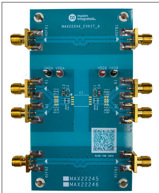
Figure 2. MAX2224XW EV Kit
