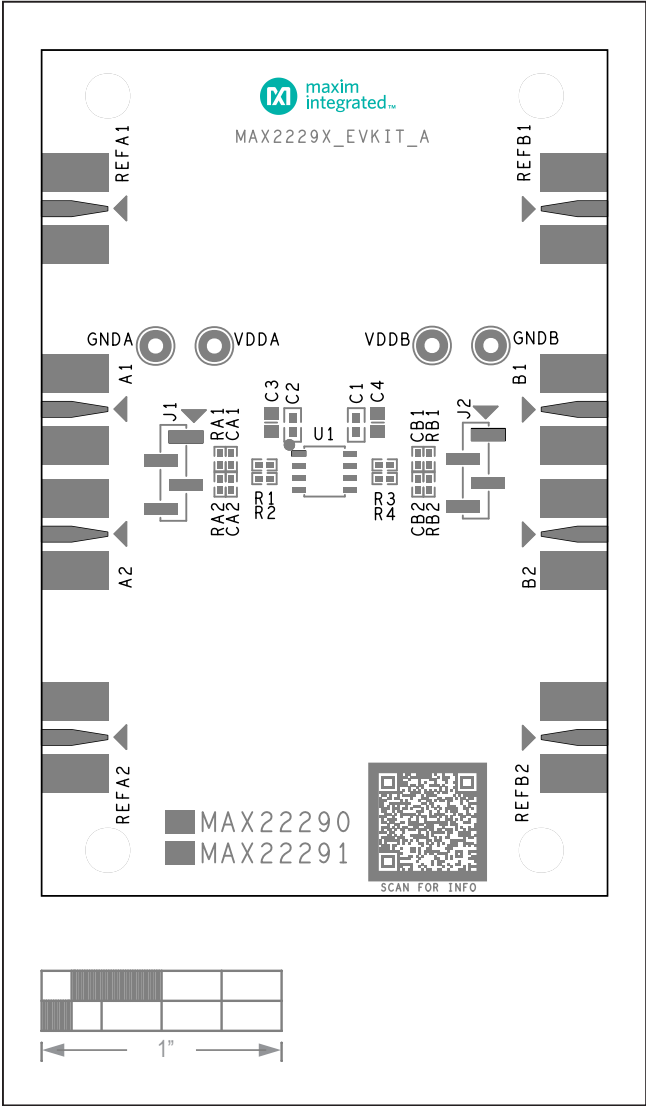
MAX22290/MAX22291 EV Kit—Top Silkscreen
