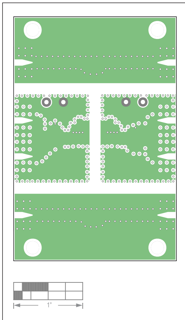
MAX22290/MAX22291 EV Kit—Layer 3 PWR
