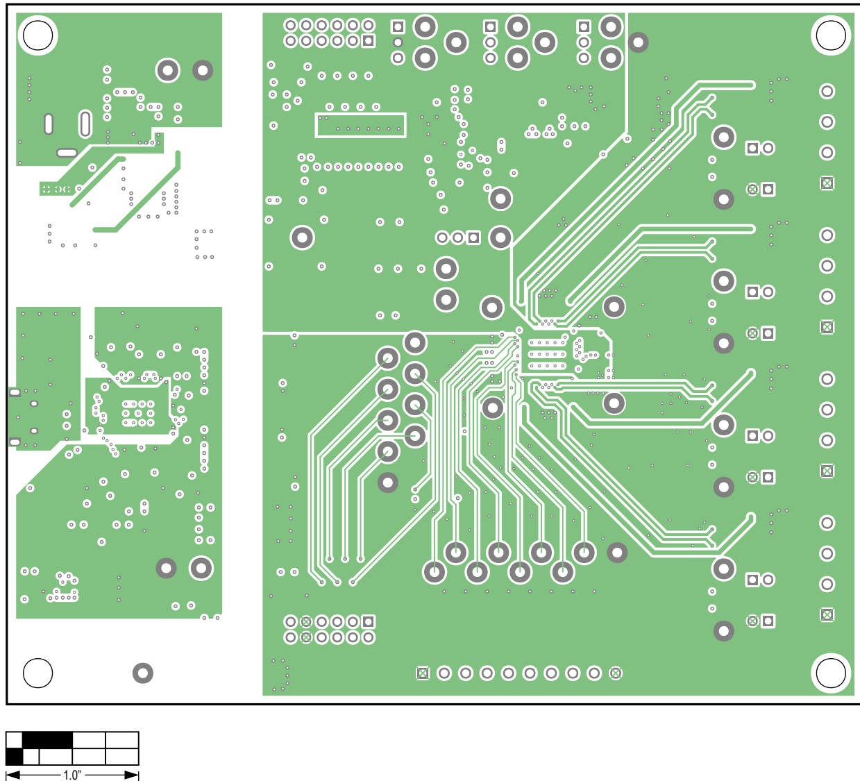
MAX22007 EV Kit PCB Layout—Layer 3
