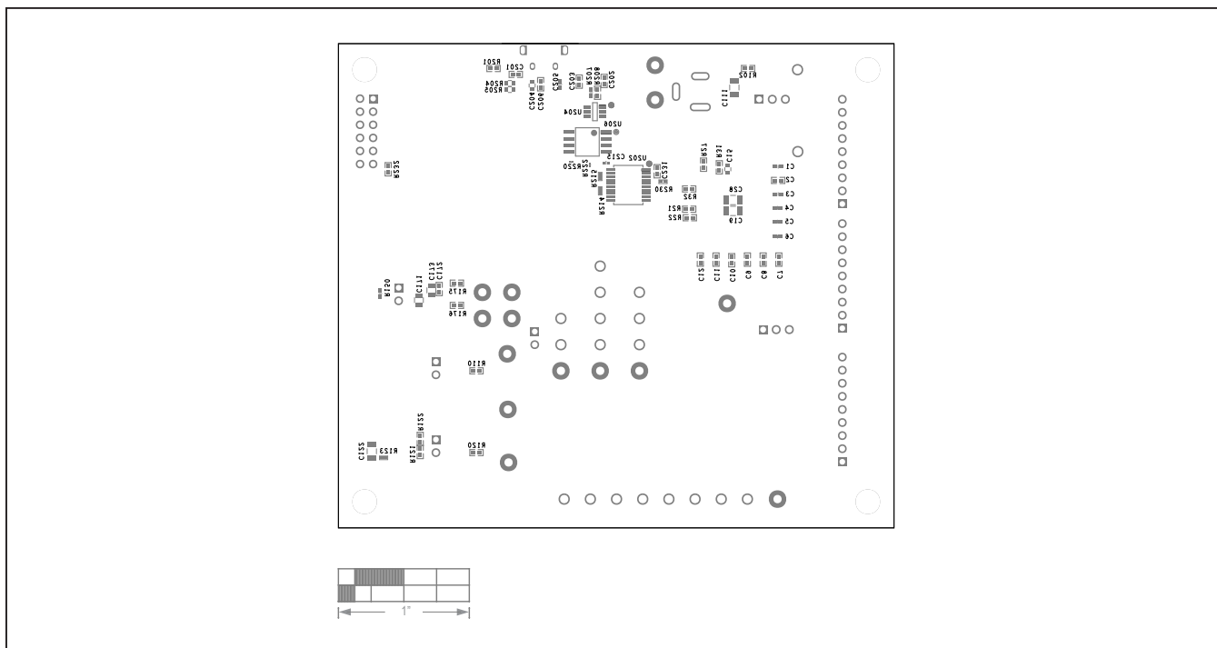
MAX22005 EV Kit PCB Layout—Silkscreen Bottom
