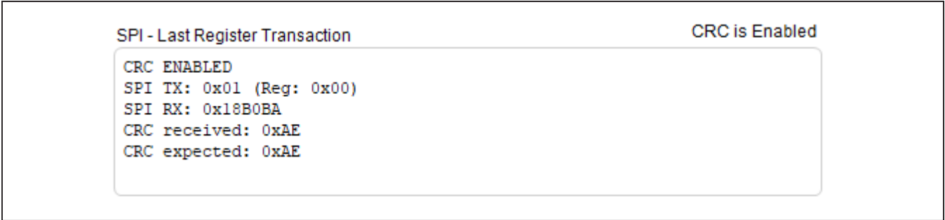
Figure 5. SPI Read Transaction with CRC Enabled
