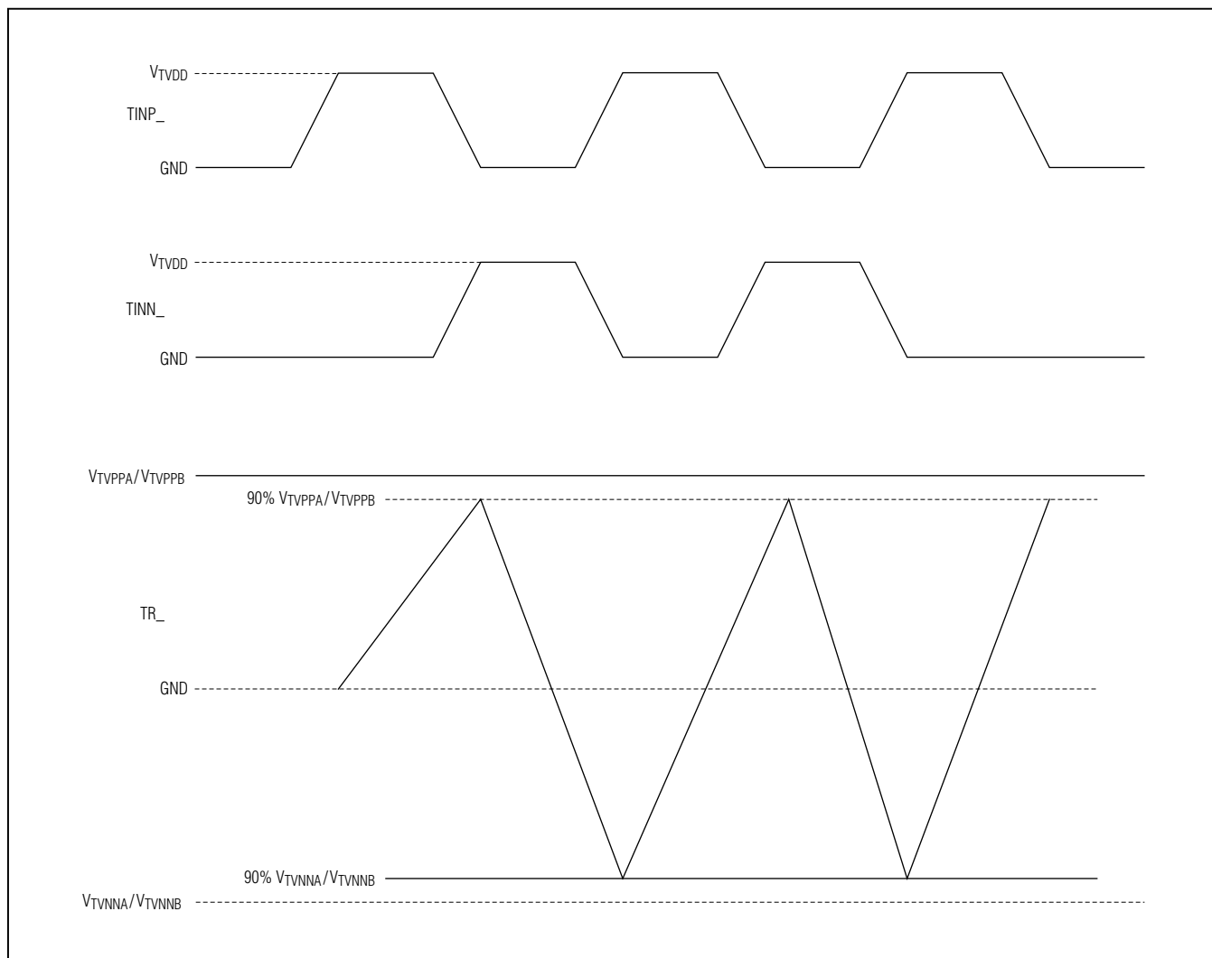
Figure 6. Bandwidth
