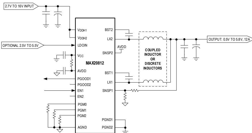
MAX20812 SINGLE-OUTPUT DUAL-PHASE APPLICATION CIRCUIT
