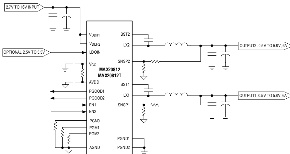
MAX20812/MAX20812T DUAL-OUTPUT APPLICATION CIRCUIT
