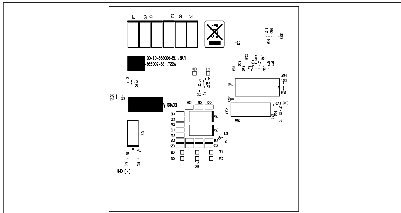
Bottom Silkscreen
